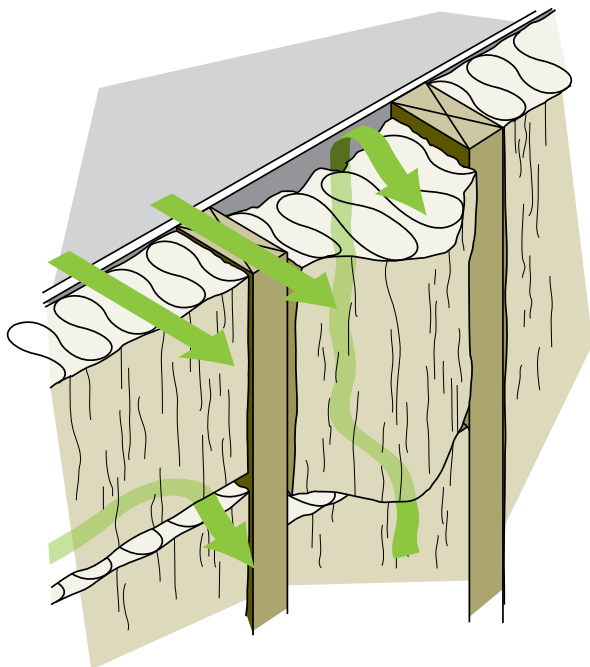
Wood studs create a thermal bridge and gaps in the insulation allow convection currents.
