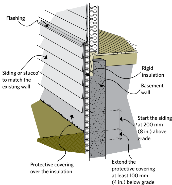
Figure 6-8 Insulating the header area from the exterior
